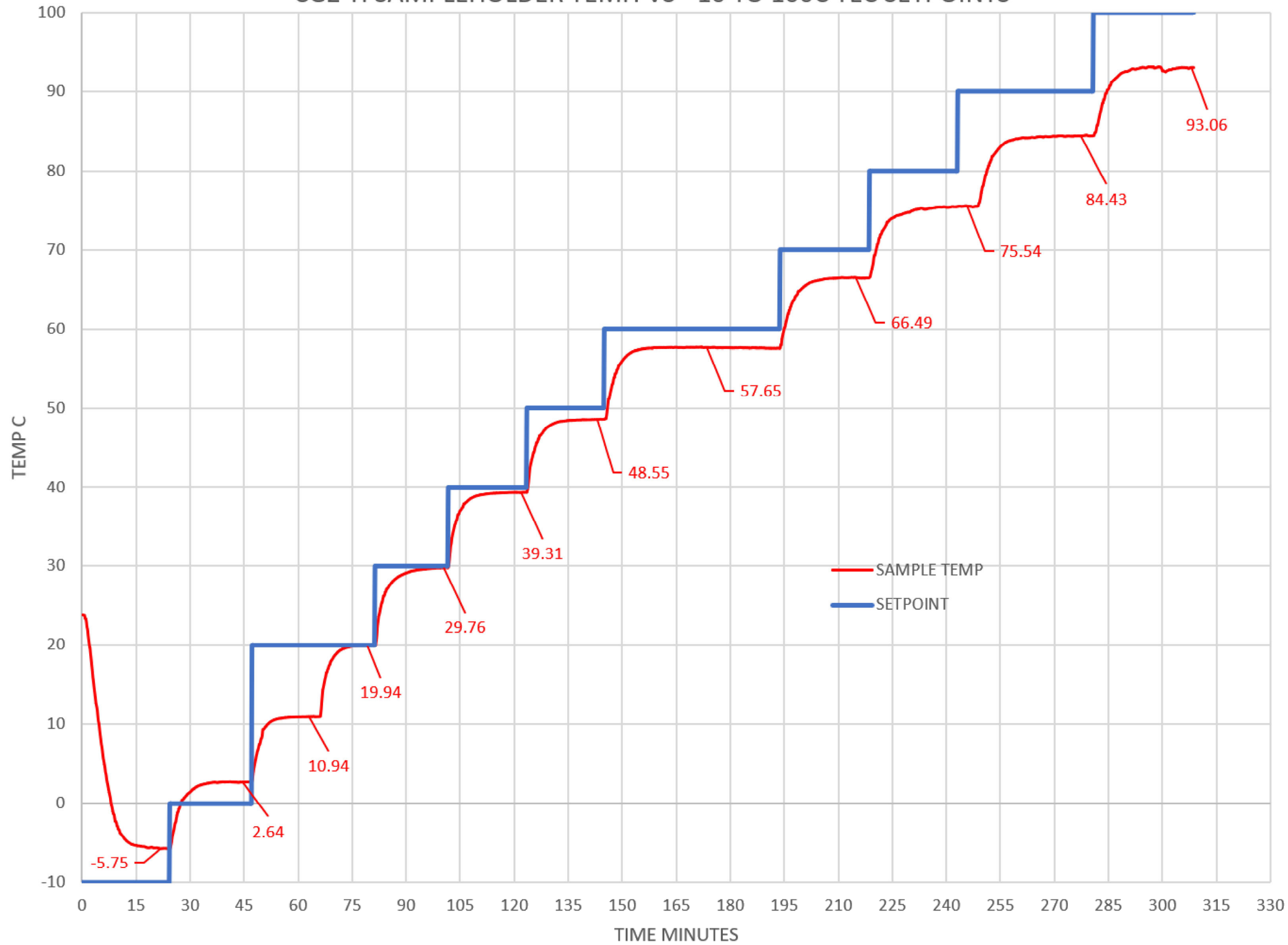
CG2 TI SAMPLEHOLDER TEMP. VS -10 TO 100C TEC SETPOINTS
